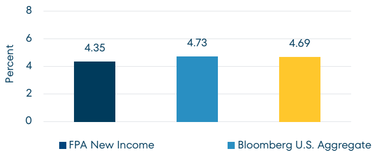
Yield-to-Worst (%)
