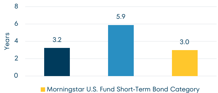
Duration (Years)
