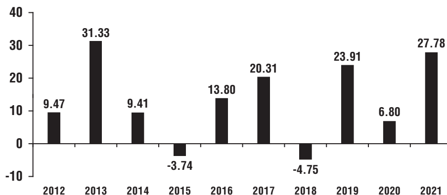
Performance Bar Chart Calendar Years Ended December 31
